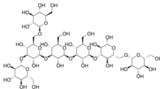
\beta -(1,3-1,6)-glucan
