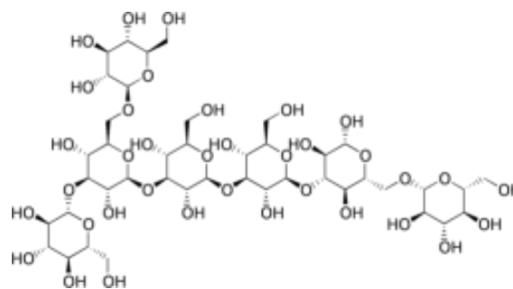
β-(1,3-1,6)-glucan
